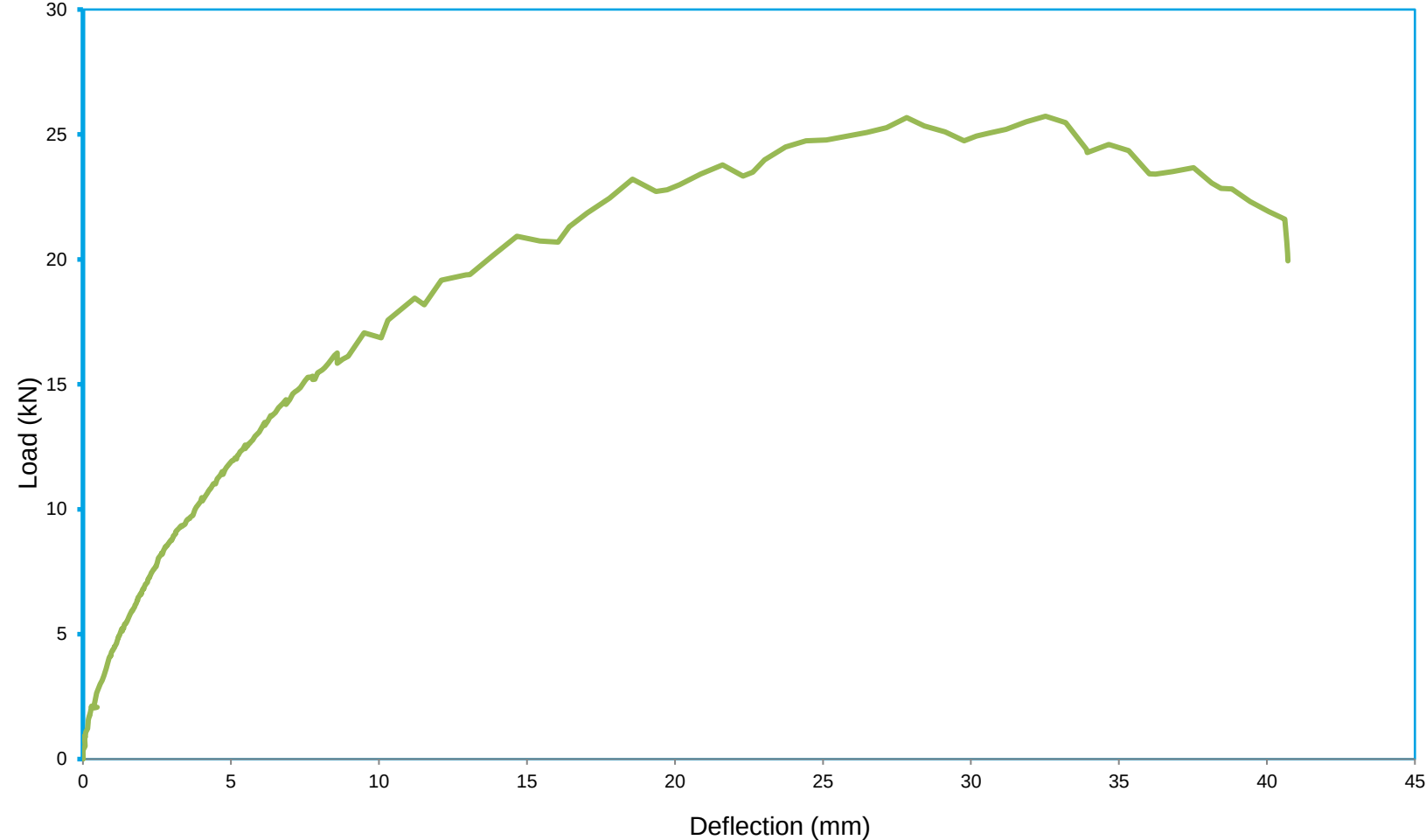
Chart 1 - Load-Deflection Curve for Racking Tests on 9 mm Magply Sheathing Boards with 50/150 mm Nailings with 0 kN Top Load
