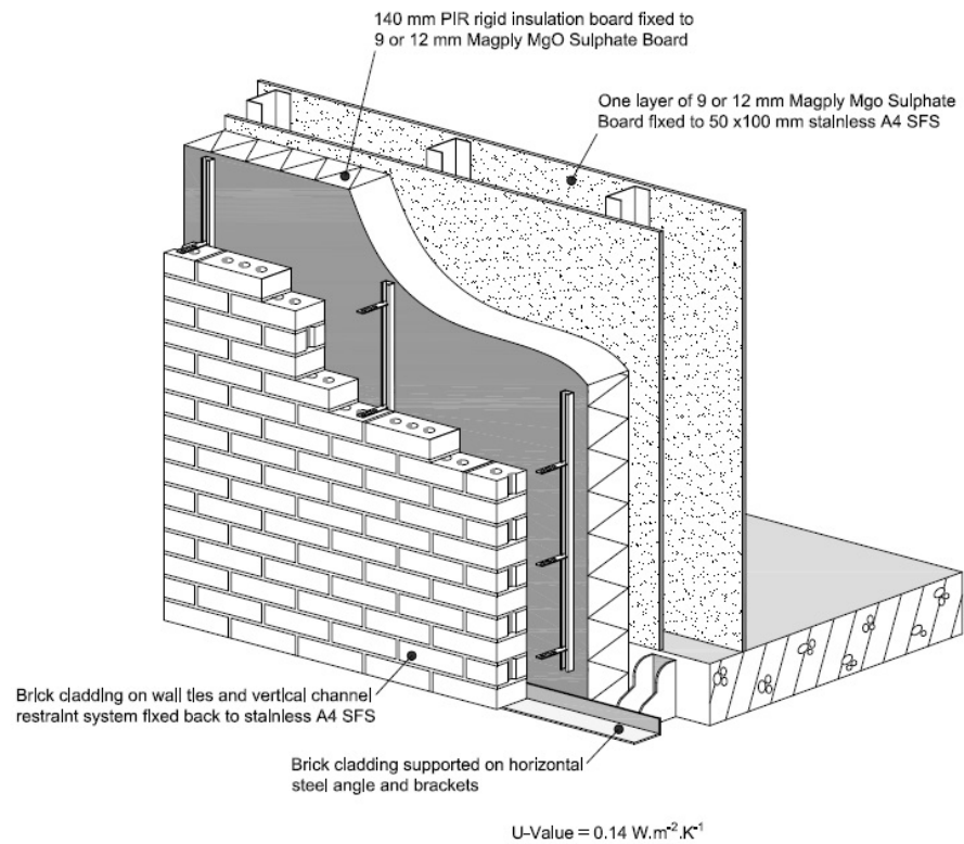
Figure 2 – typical example 2 of internal lining to finished external walls
