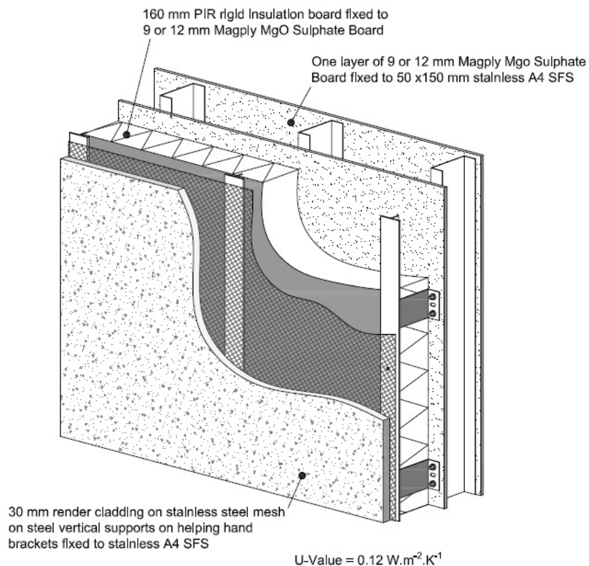
Figure 3 – typical example 3 of internal lining to finished external walls
