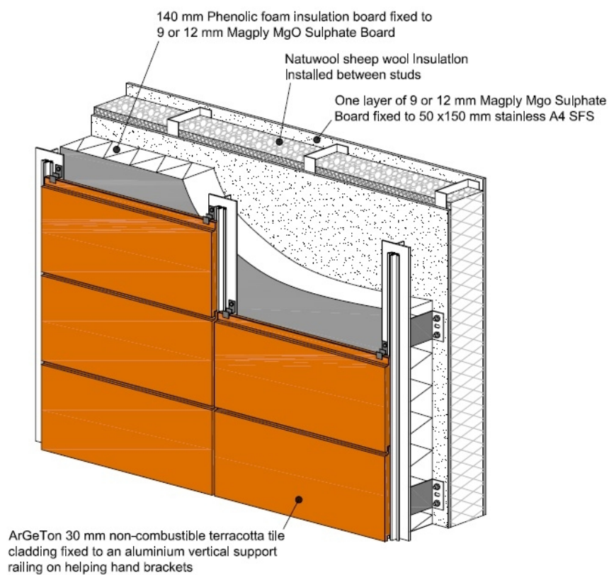
Figure 4 – typical example 4 of internal lining to finished external walls
