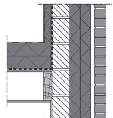
Warm roof
