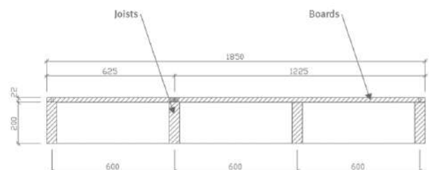
Diagram 4 - section of particleboards fixed at 600 mm joist centres
