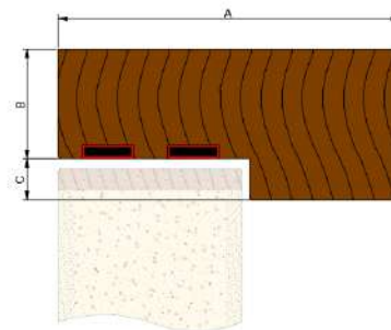
Standard Rebated Transom/Mullion Detail (modular framing)
